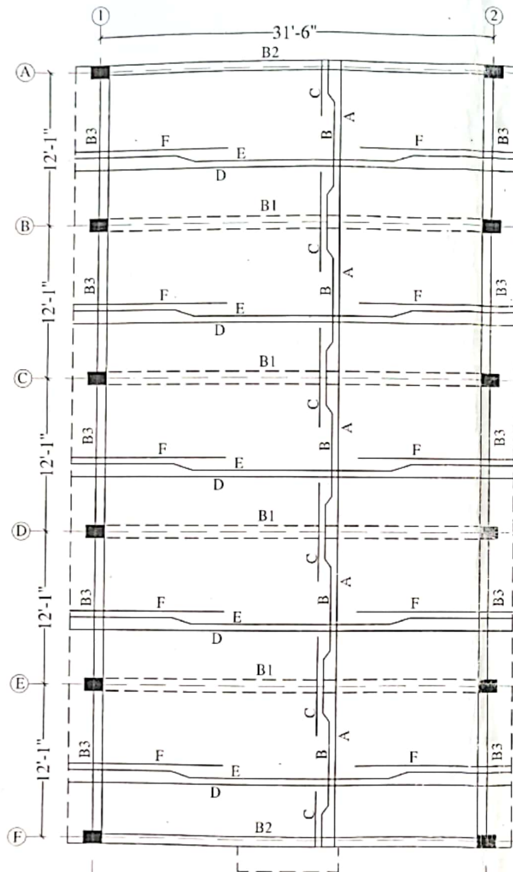
GROUND FLOOR ROOF BEAM & SLAB LAYOUT PLAN
