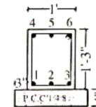
PLINTH BEAM 'PB2'
