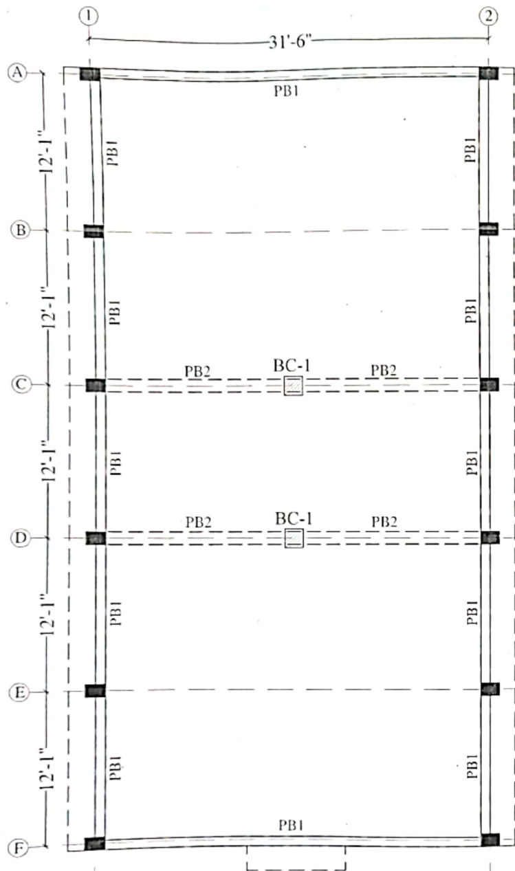
PLINTH BEAM LAYOUT PLAN
