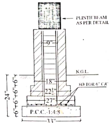
SECTION AT B-B
