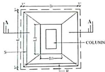
TYPICAL PLAN OF COLUMN FOOTING
