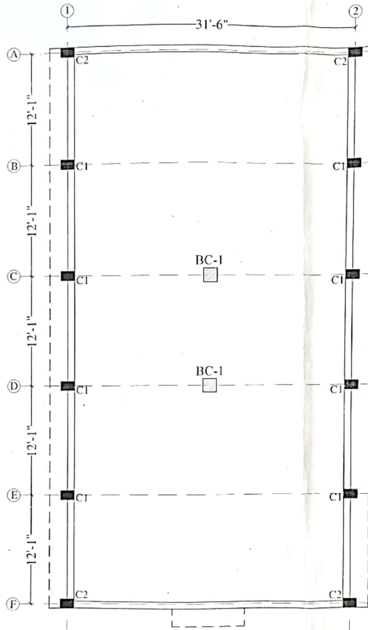
COLUMN LAYOUT PLAN
