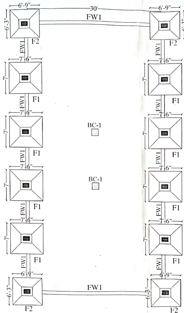
FOUNDATION LAYOUT PLAN
