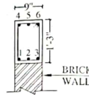
PLINTH BEAM 'PB1'
