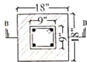
BAR NO. :- 1 TO 4 - 160 TOR RINGS:- 80 TOR @ 6" C/C THROUGHOUT COLUMN BC-1 (18" X 18")
